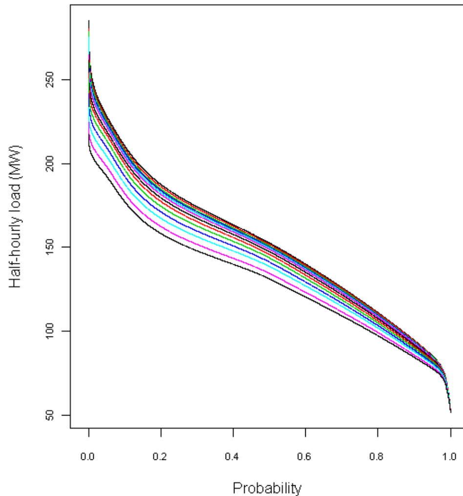
Load probability curves (ANNUAL): NelsonMarlborough
