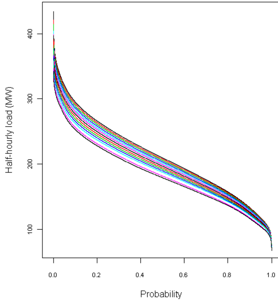
Load probability curves (ANNUAL): Central
