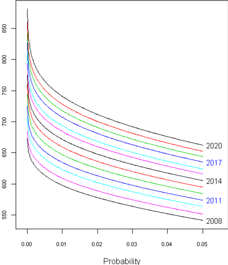
Load probability curves (ANNUAL): Wellington
