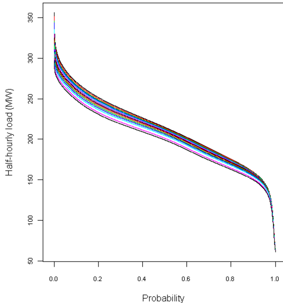
Load probability curves (ANNUAL): HawkesBay
