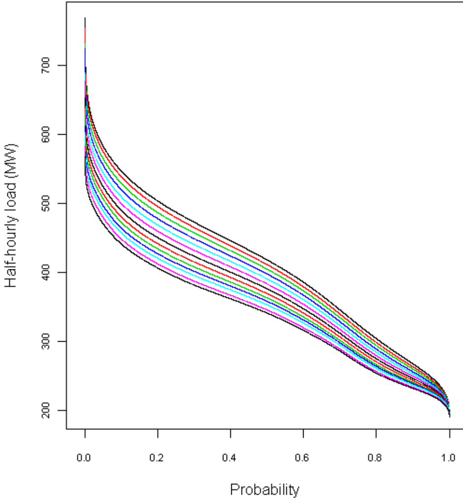
Load probability curves (ANNUAL): Waikato
