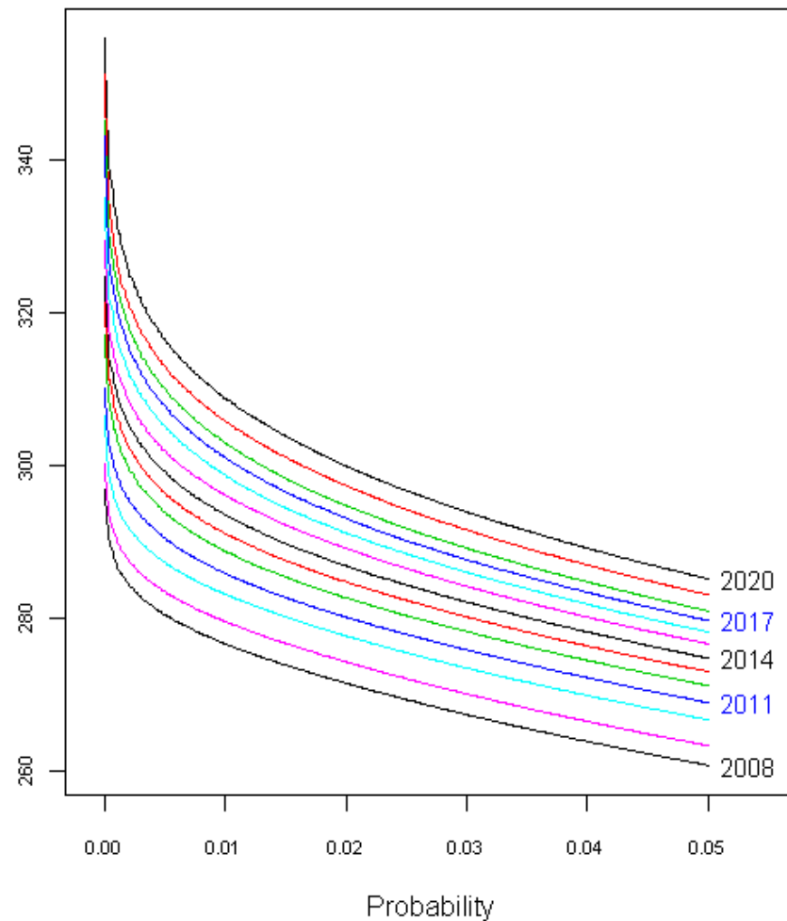
Load probability curves (ANNUAL): HawkesBay
