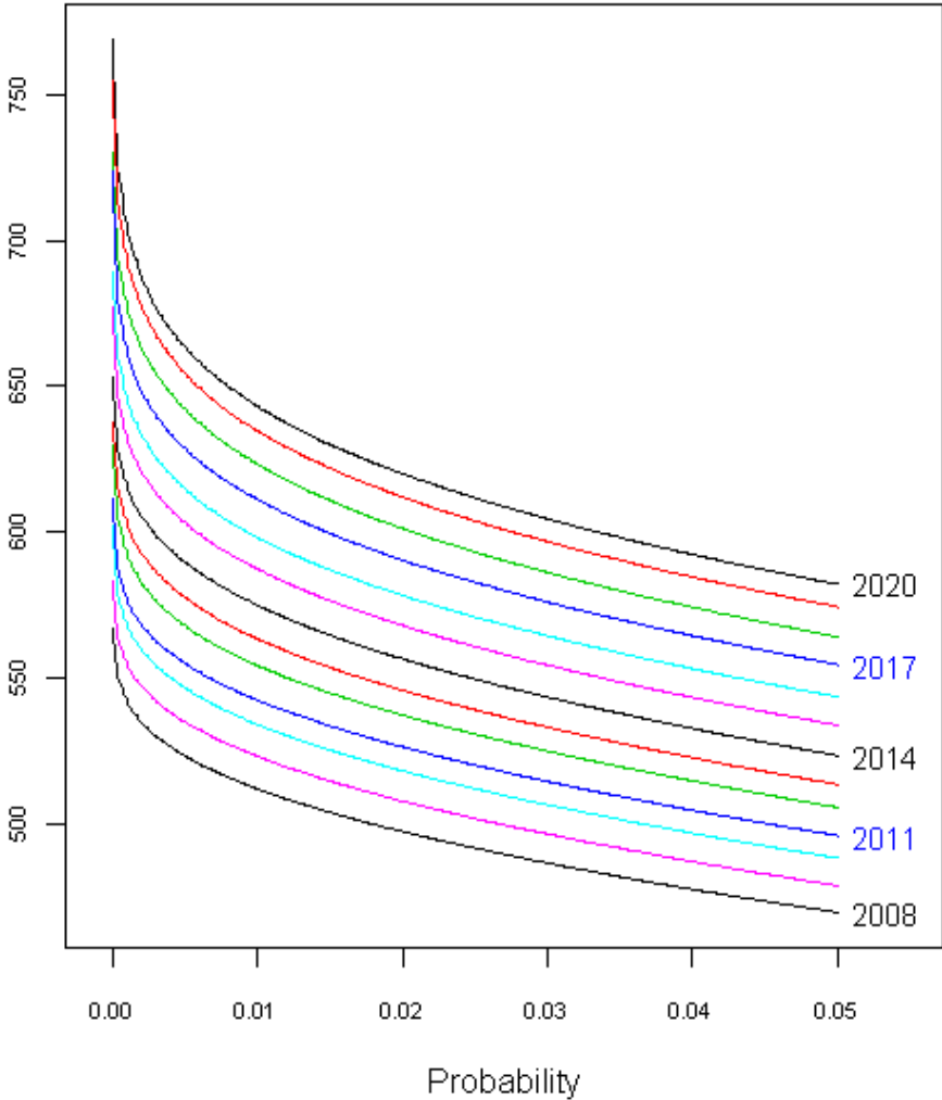
Load probability curves (ANNUAL): Waikato
