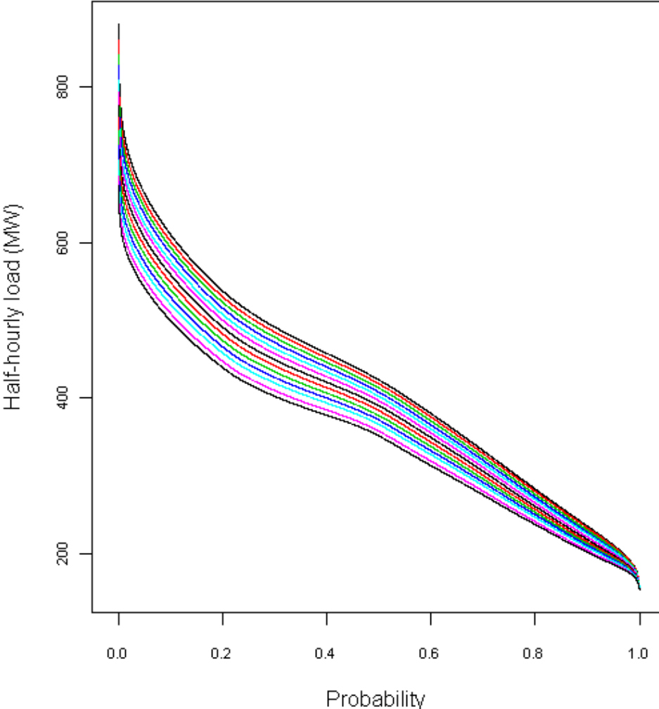
Load probability curves (ANNUAL): Wellington
